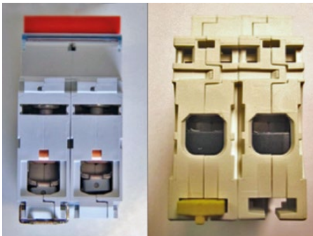
Fig 12. Cable entries of main-switches showing tabs below moving part of terminal – as design feature to minimise the likelihood placing conductors in terminal incorrectly
