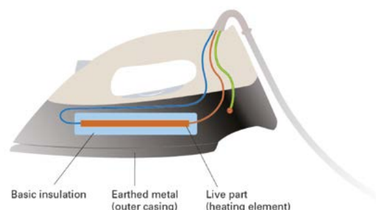
Fig 2. Class I equipment construction
