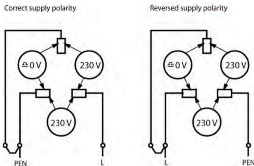
Fig 1. Reversal of polarity in the supply in a TN-C-S system
