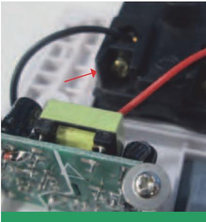
Fig 2. Soldered connections in the accessory prevented the test plug being fully inserted
